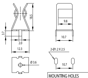
CQ-216(G) For 10.3mm Dia. Fuse
