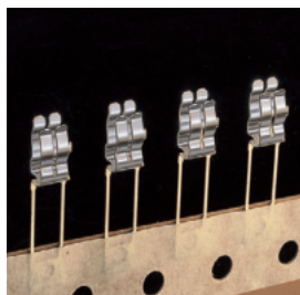
CQ-05CT Tape/Reel For 5mm Dia. Fuse
