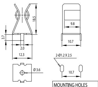
CQ-216 For 10.3mm Dia. Fuse
